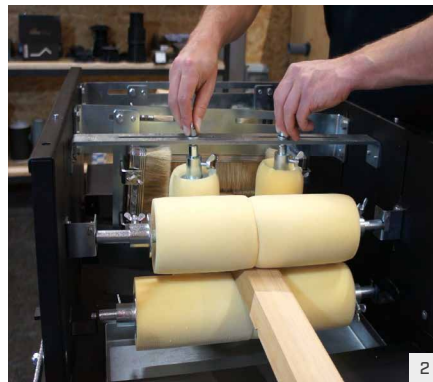
2 Adjust the sponges to the dimensions of the element and fix them by tightening screws.
