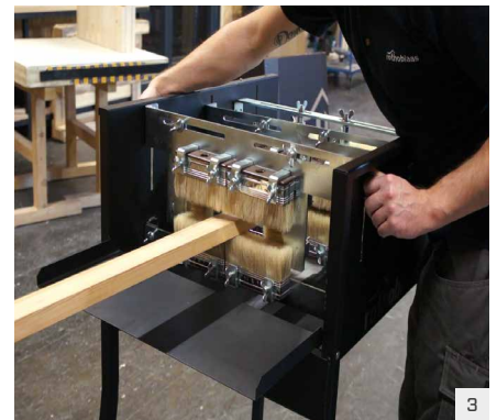
3 Adjust the brushes to the dimensions of the element and fix them by tightening screws.
