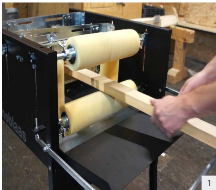
1 Insert the element between the two automatic coating machines
